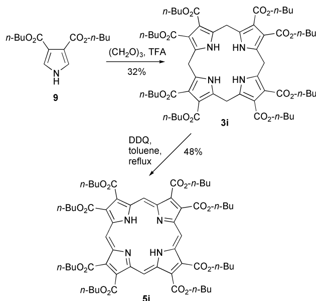
Scheme 3 Cyclo-oligomerization of dibutyl pyrrole-3,4-dicarboxylate.
